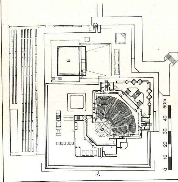
Plan, level 4 (Olivier circle)
