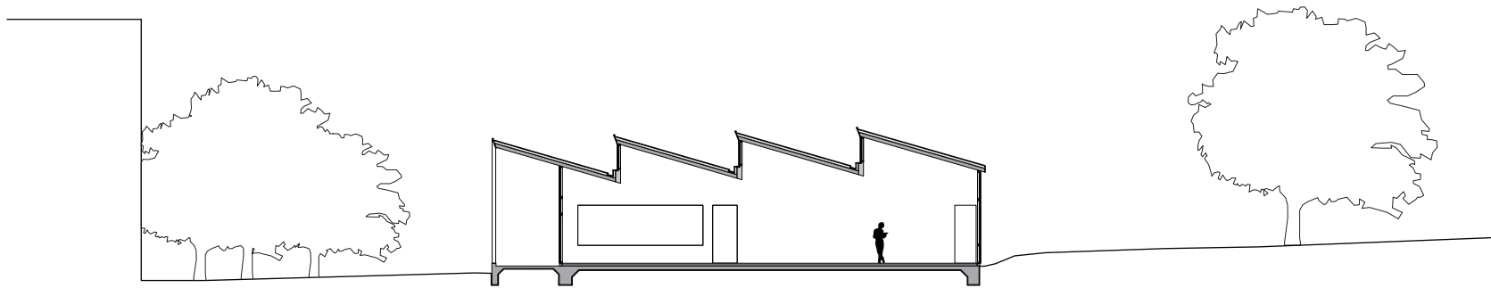
Short Section - North/South
