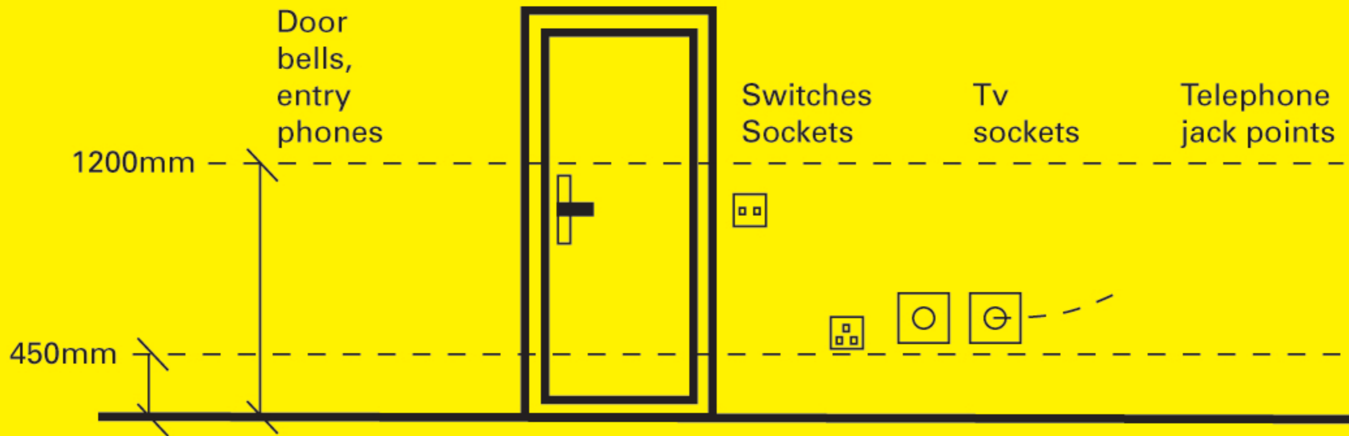
Guideline appliance heights under Part M.
