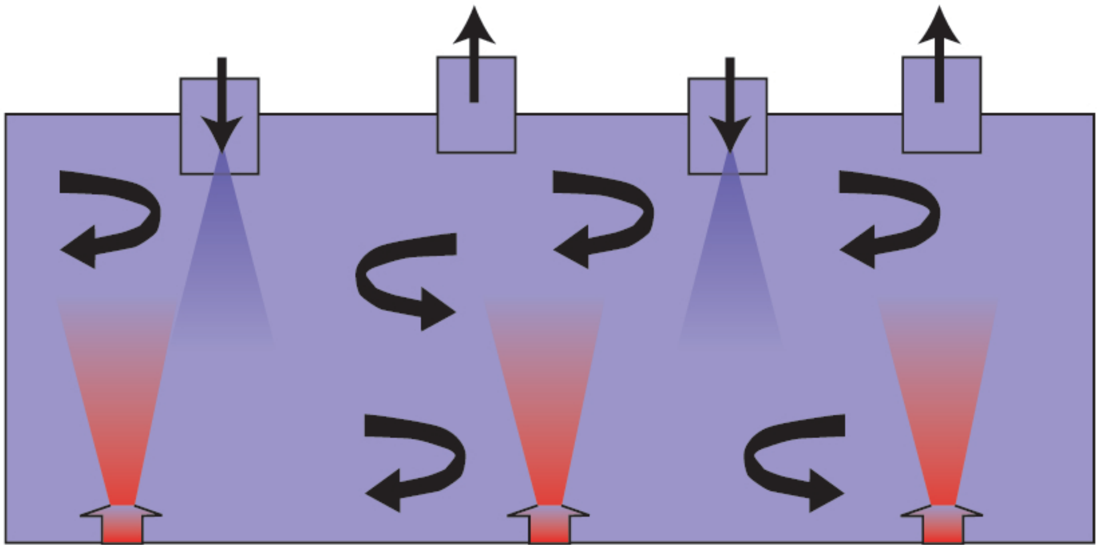
Figure 5. The flow pattern which can develop in a mixing ventilation system in which cold inflowing air descends from a series of roof stacks and mixes and dilutes prior to reaching the floor of the space, while a series of localised heat sources produce upflowing plumes of warm air which mix with interior air in upflowing plumes. There is an outflow of warm interior air which matches the inflow of cold exterior air
