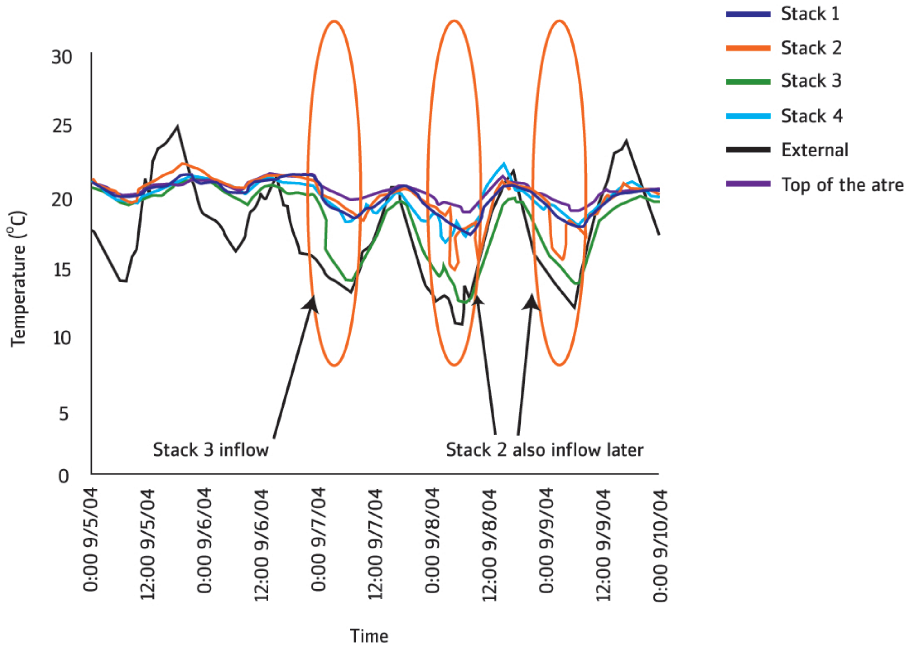
figure 2. Time series of the temperatures in the four stacks, the interior of the Contact Theatre at a height of 3 m above the floor, and the exterior
